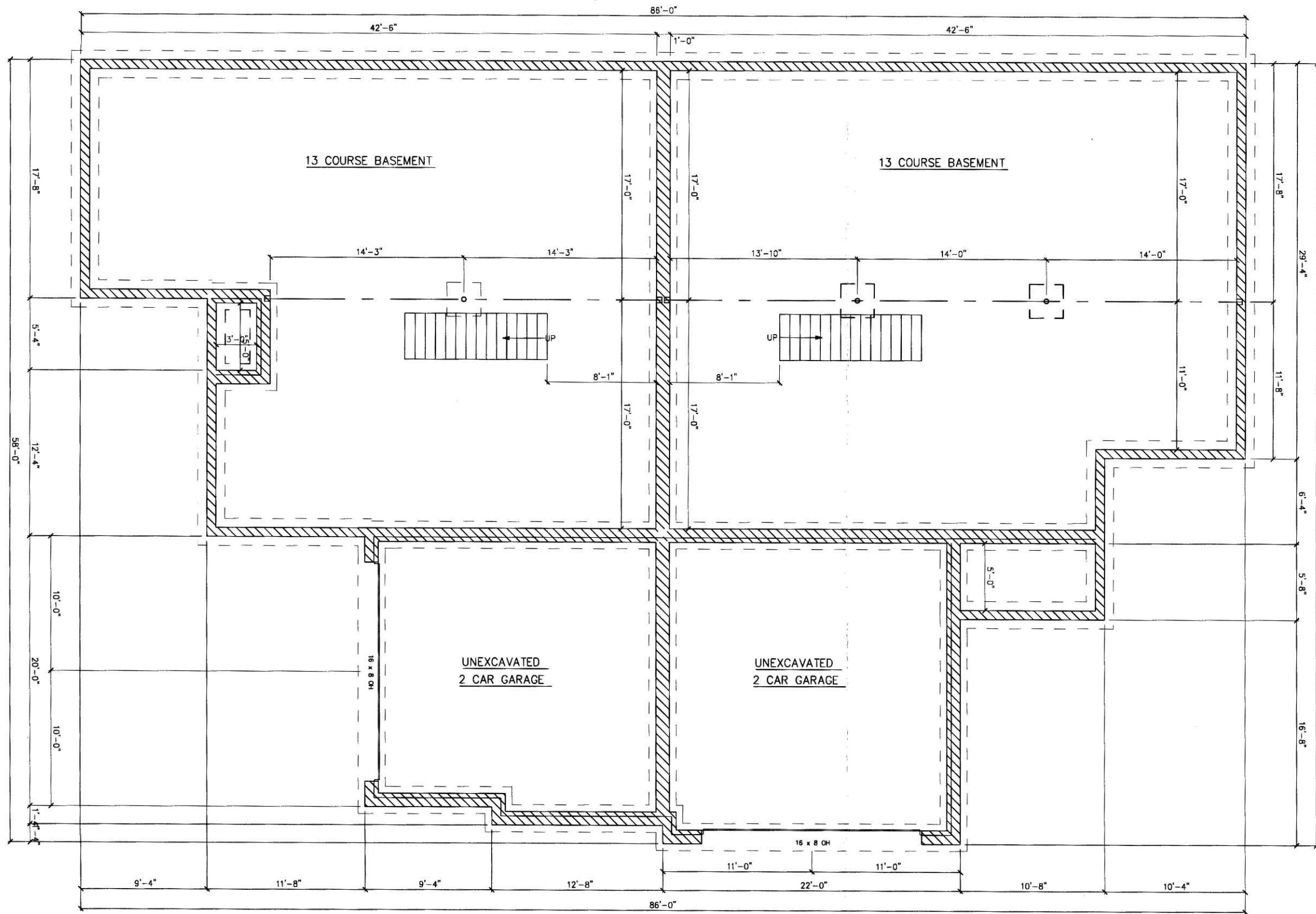
FOUNDATION PLAN
